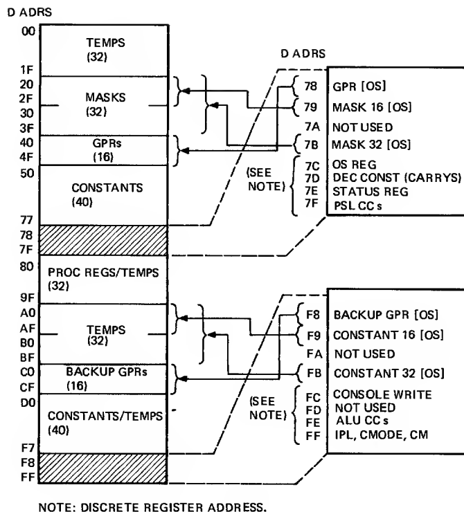
Figure 6-11 Local Store Address Assignments
